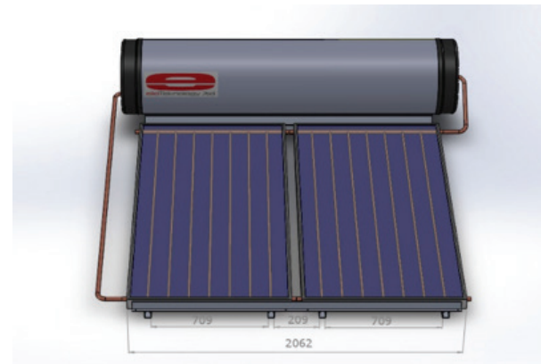
300 liters model
