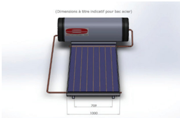
200 liters model
