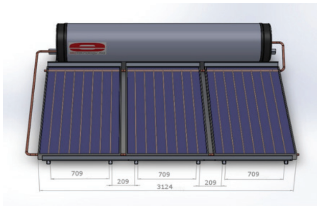
400 liters model
